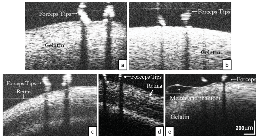
Fig. 7. Real-time B-scan OCT imaging examples for the OCT-guided conditions. (a) Manual B-scan OCT-forceps approaching gelatin phantom (Media 6). (b) Robot-assisted B-scan OCT-forceps approaching gelatin phantom (Media 7). (c) Manual B-scan OCT-forceps approaching goat ex vivo retina (Media 8). (d) Robot-assisted B-scan OCT-forceps approaching goat ex vivo retina (Media 9). (e) Real-time B-scan OCT imaging of peeling membrane phantom from gelatin (Media 10)
